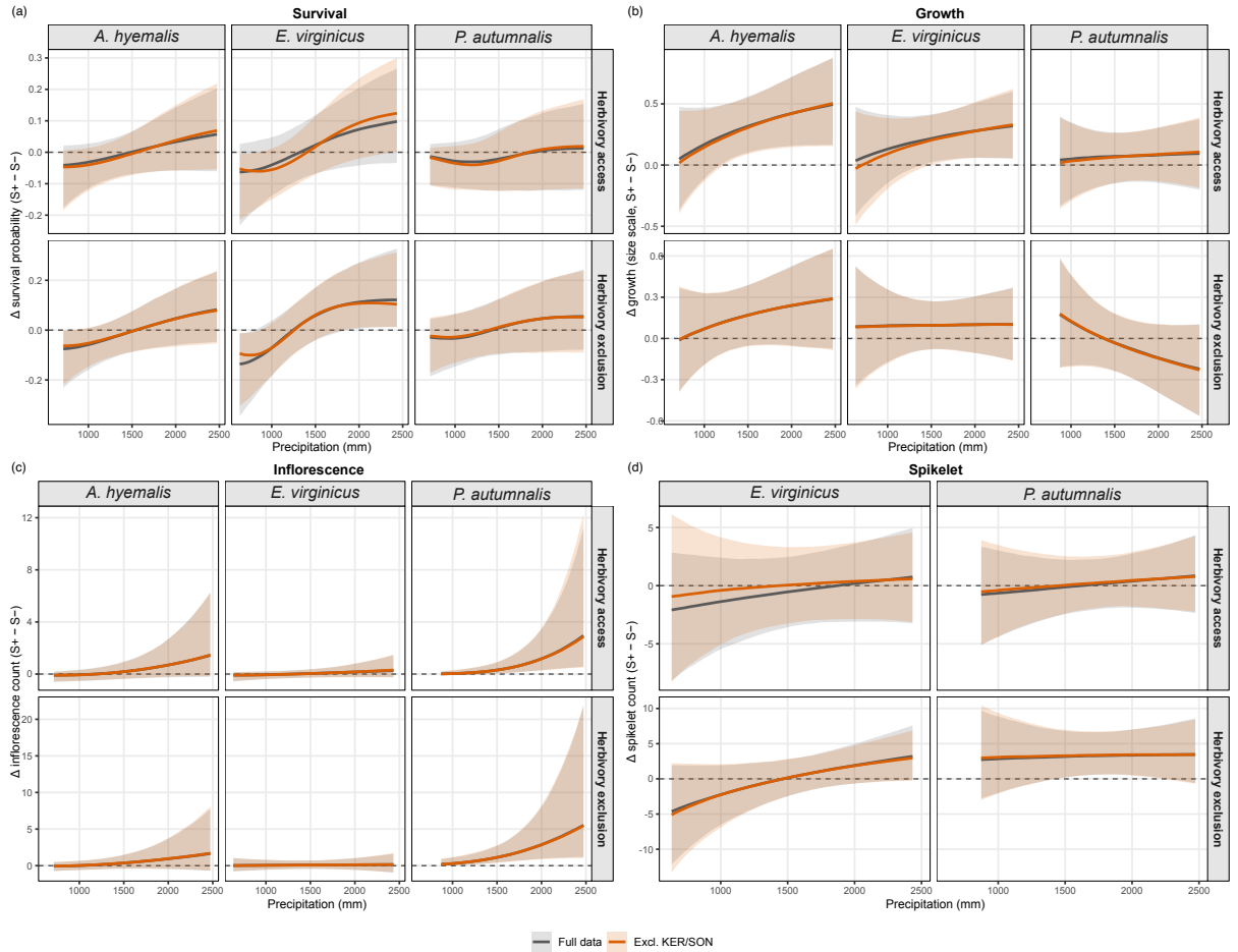
Figure S6: Posterior median (line) and 90% credible interval (shading) of endophyte effects ( \Delta = S^+ - S^- ) for the full dataset (gray) and for the dataset excluding KER and SON (orange), by vital rate, species, and herbivory treatment.
